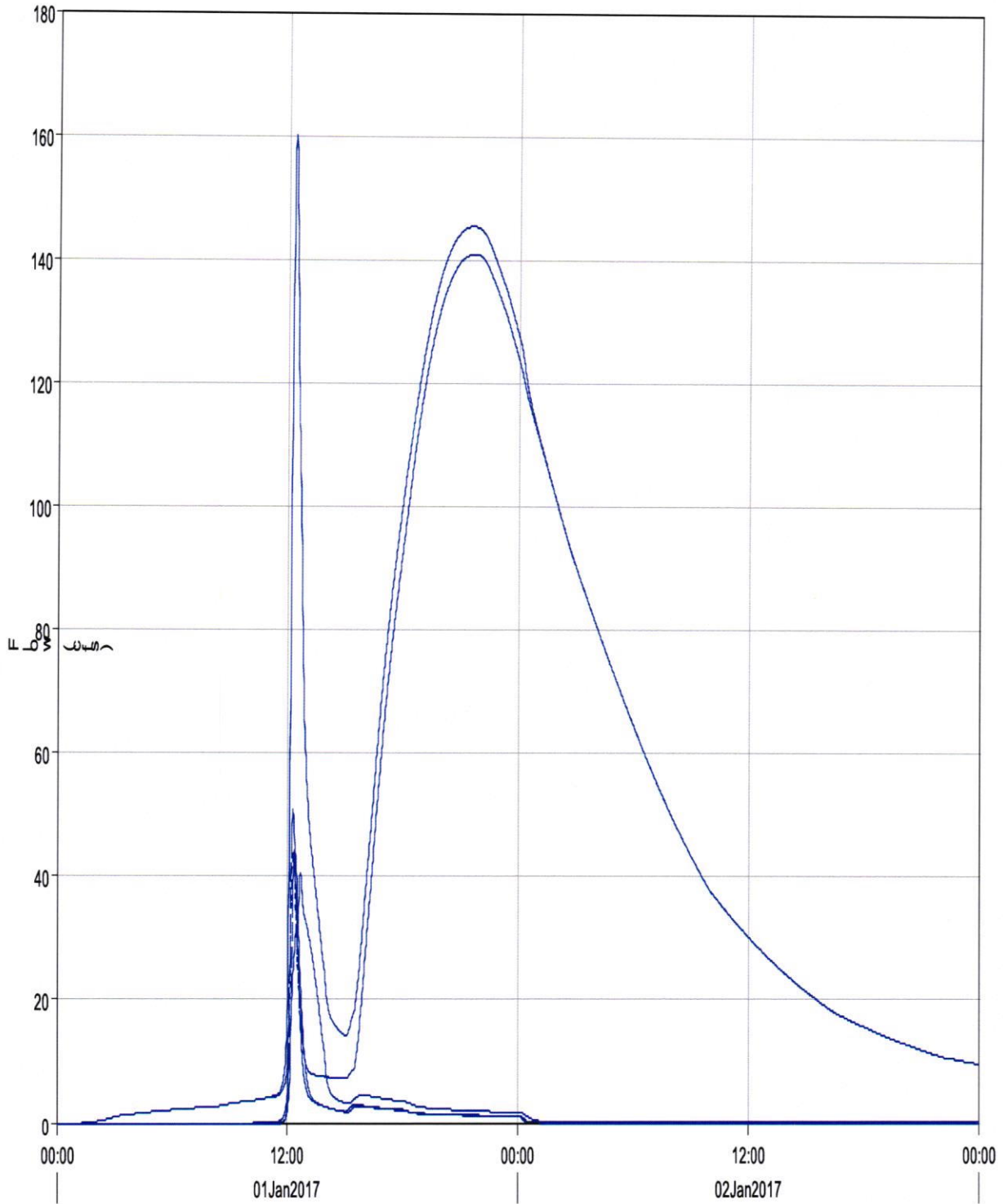
Junction "PointC" Results for Run "Proposed_100year"
