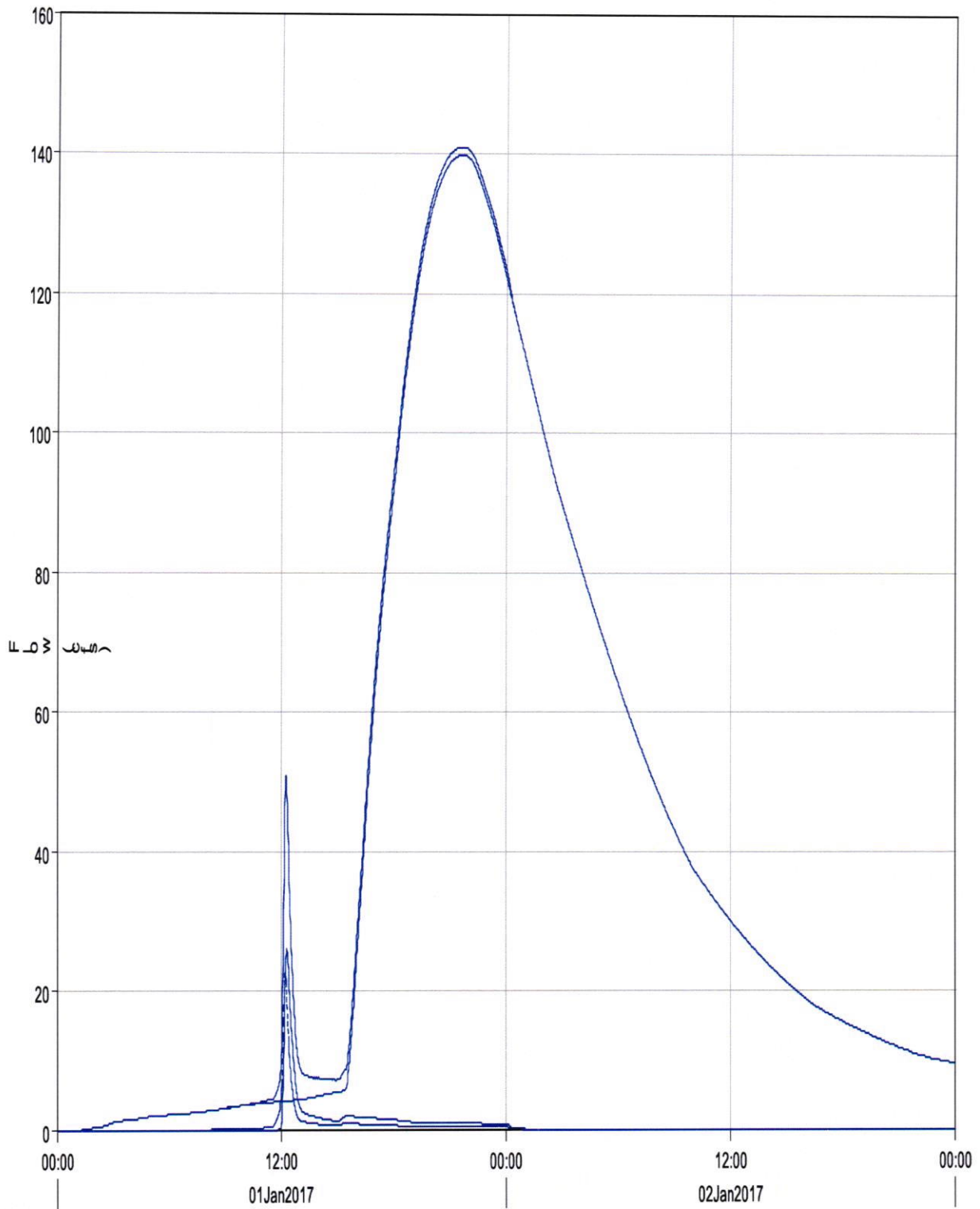
Junction "PointA" Results for Run "Proposed_100year"
