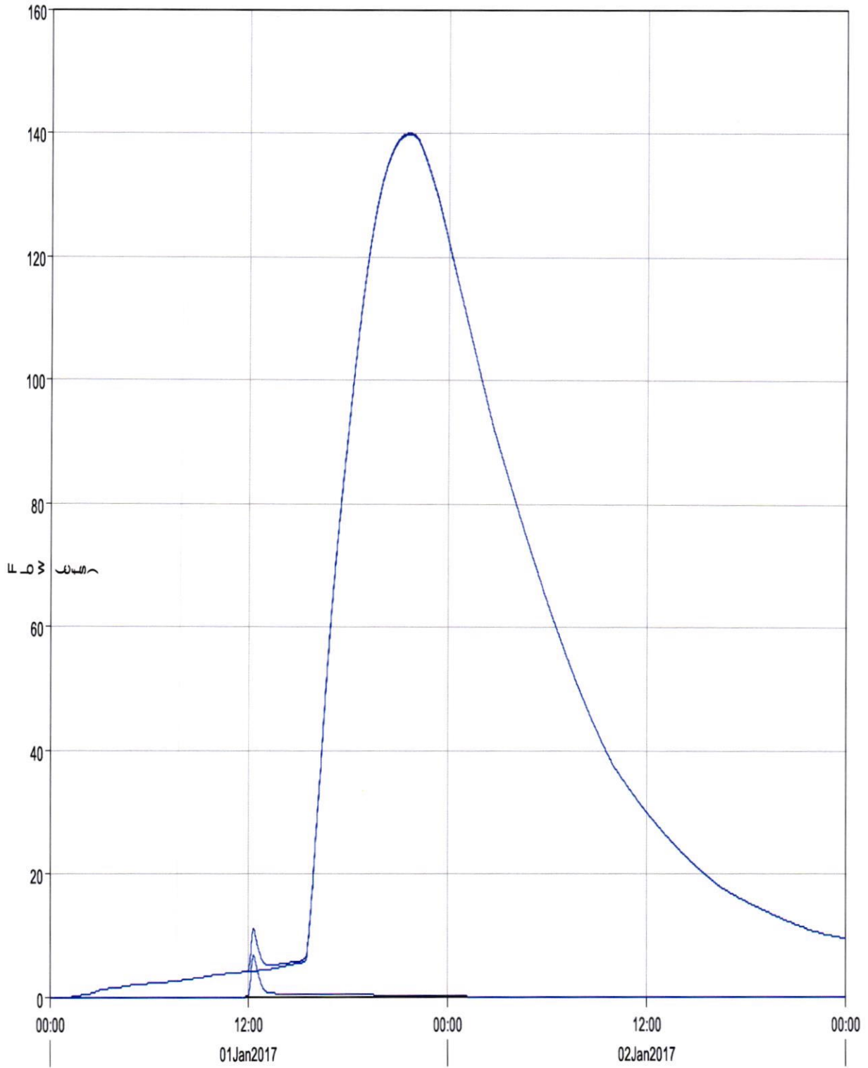
Junction "PointA" Results for Run "Existing_100year"
