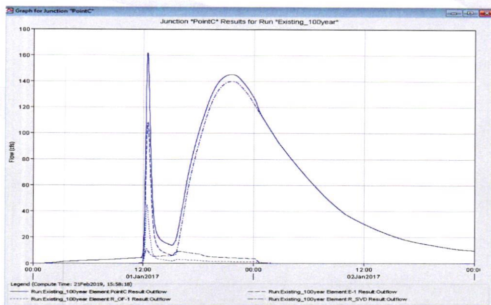
Figure 2 - Existing Hydrograph at Confluence Point C
