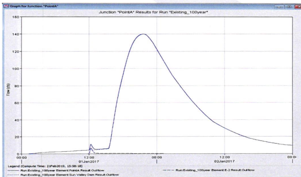
Figure 1 - Existing Hydrograph at Confluence Point A
