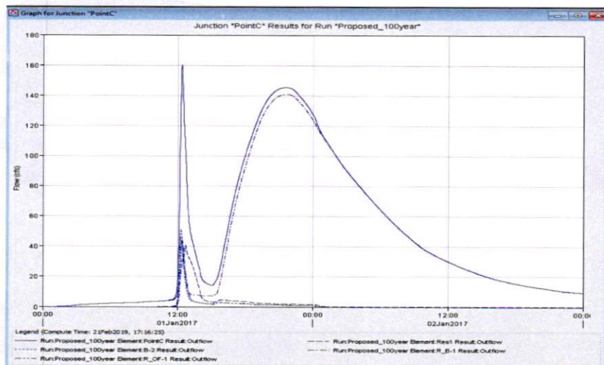
Figure 3 -Proposed Hydrograph at Confluence Point C
