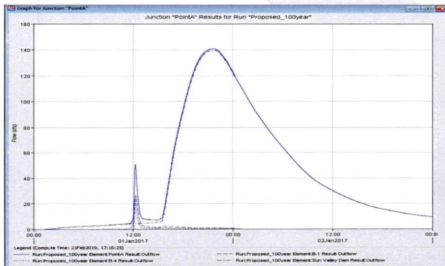
Figure 2 -Proposed Hydrograph at Confluence Point A
