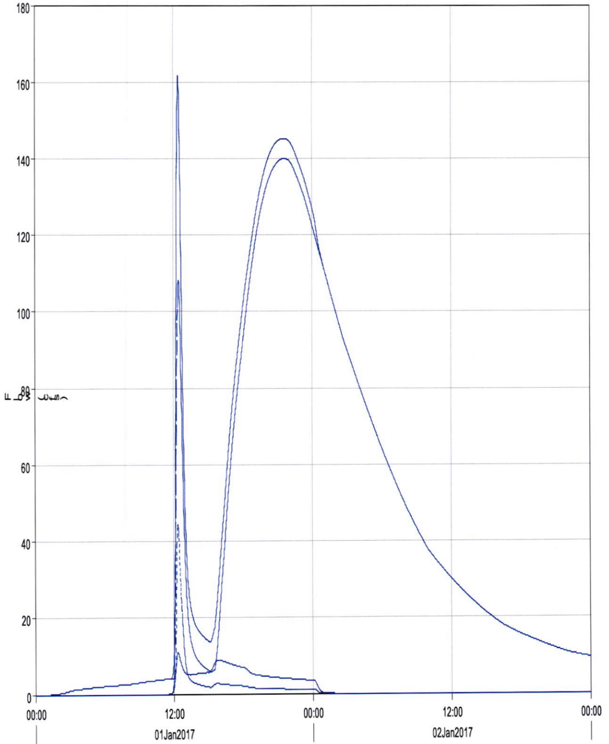
Junction "PointC" Results for Run "Existing_100year"
